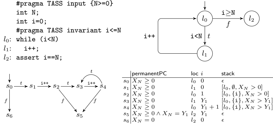
Fig. 2. A simple example to prove an assertion for all values of N . Top: source code with TASS annotations and program graph. Bottom: the reachable state space in the loop transition system; t represents the true branch and f the false branch.
