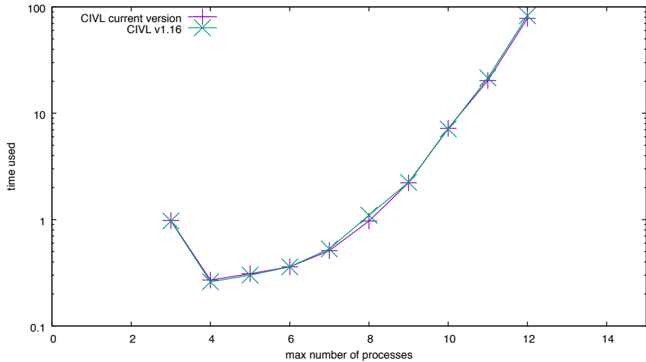
Dining philosopher verification time
